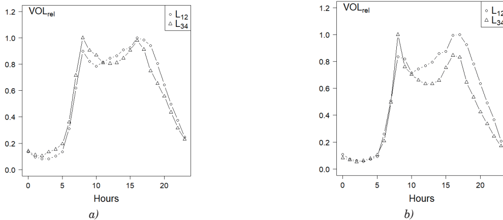
Figure 13 Relation between the relative annual hourly traffic volume and time for 24 h period at weekdays on entry lanes ( L_{12} ) and exit lanes ( L_{34} ) from the city a) in 2011, b) in 2016
