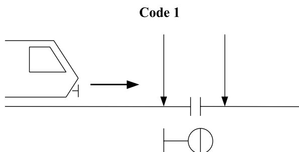
Fig. 3 Supply of the track circuits before and behind the signal
