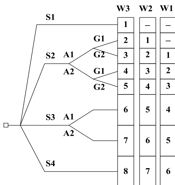
Fig. 2 Risk graph
