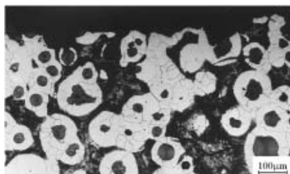
E 144, T = 20\text{ }^{\circ}\text{C} , KCV = 5\text{ J/cm}^2
