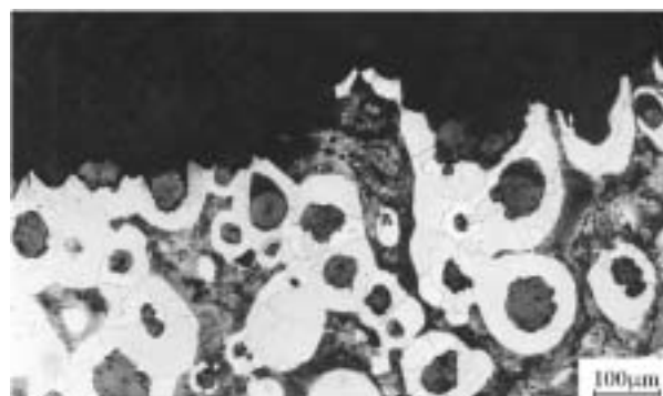
E 171, T = 100\text{ }^{\circ}\text{C} , KCV = 14.6\text{ J/cm}^2
