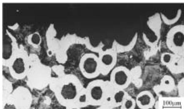
E 144, T = 140\text{ }^{\circ}\text{C} , KCV = 15.4\text{ J/cm}^2
