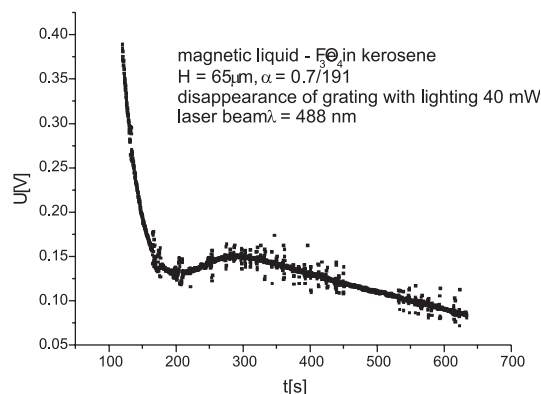
Fig. 2 The time dependence of decay of the lighting particles grating when S < 0 .
