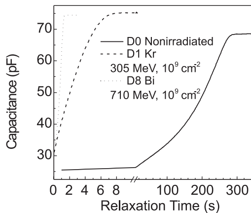
Fig. 3. MOS structures D0, D1, D8 measured C-t curves of MOS structure before and after irradiation by Kr and Bi ions with the same fluence 10^9 \text{ cm}^{-2}
