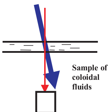
Fig. 4 Schematic arrangement for reading data to determine the light absorption in the sample.
