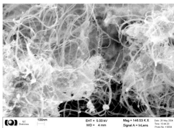
Fig. 2 Carbon nanotubes grown on non-conducting substrates magnified a) 146 530 x and b) 5 970 x
