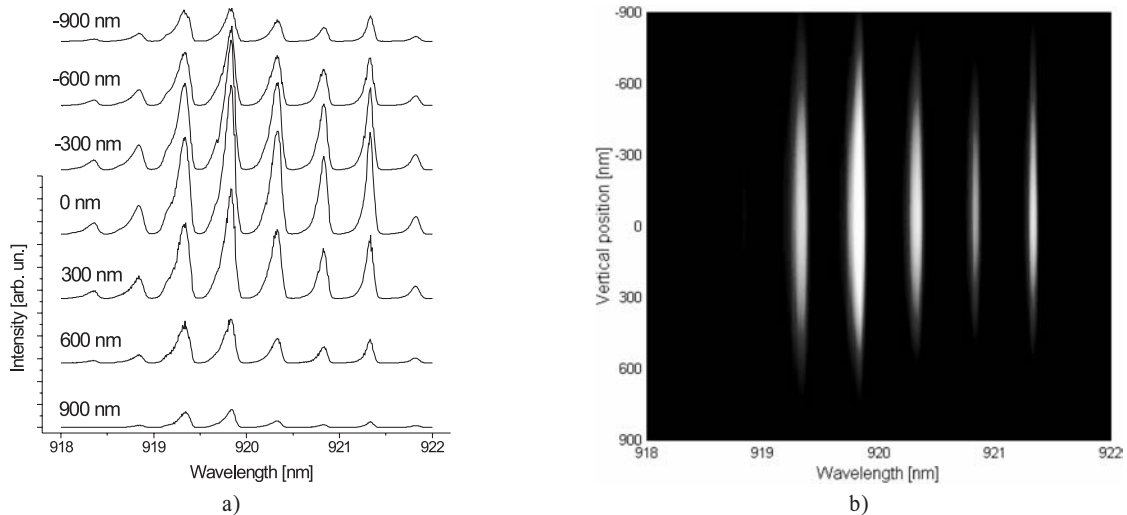
Fig. 6 a) Laser mode spectrum at different vertical positions of the fiber tip at driving current I = 50 mA, b) interpolated density image.
