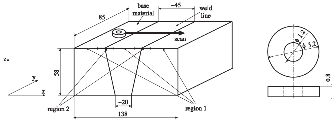
Fig. 2 Configuration and dimensions of the specimen and the pancake probe
