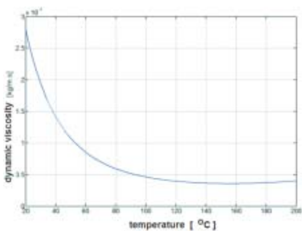
Graph 2. Dynamic viscosity
