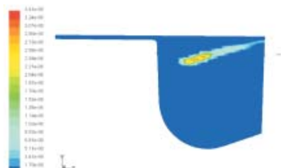
Fig. 31 Droplets of ethanol 0 °CA before TDC, kinetic model
