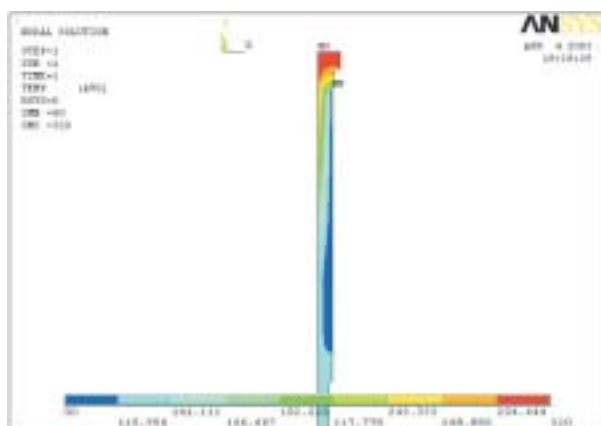
Fig. 6 Results of heat transfer in C°
