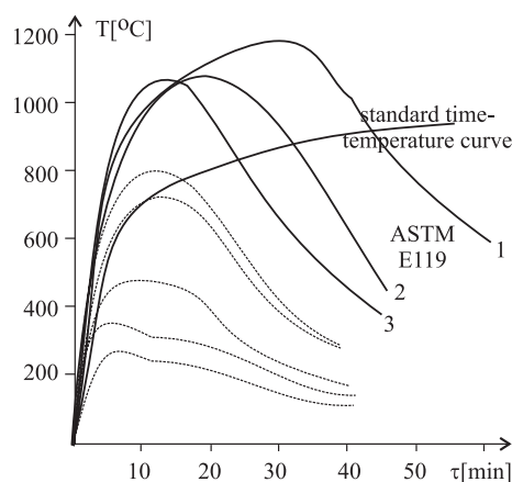
Fig. 3 ASTM E119 curves and standard time-temperature curve
