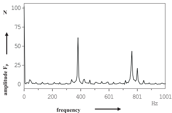
Fig. 6 Frequency - amplitude spectrum for V_o = 1500 mm 3 , a_p = 0.03 mm A99 grinding wheel
