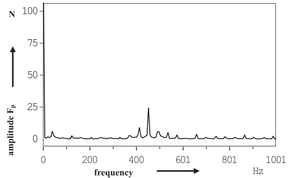
Fig. 7 Frequency - amplitude spectrum for V_o = 1500 mm 3 , a_p = 0.03 mm 5SG grinding wheel
