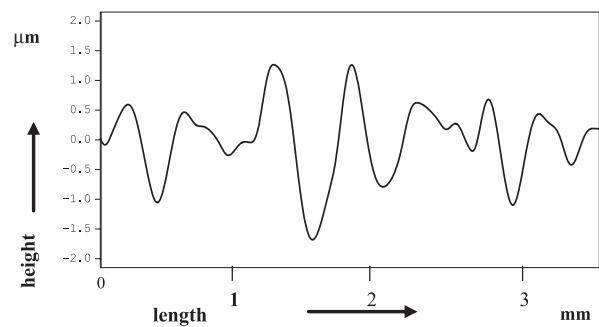
Fig. 8 Waviness of ground surface generated by conventional Al_2O_3 wheel, a_p = 0.03 mm, V_o = 1170 mm 3
