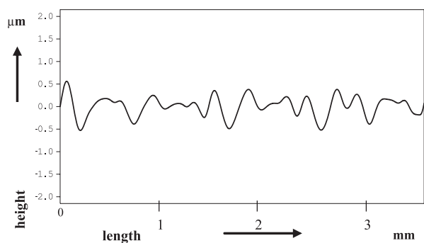
Fig. 9 Waviness of ground surface generated by 5SG wheel, a_p = 0.03 mm, V_o = 1170 mm 3
