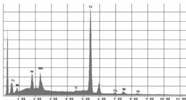
Fig. 6 EDX spectrum of the phase \text{M}_{23}\text{C}_6
