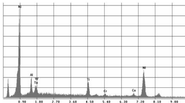
Fig. 4 EDX spectrum of the phase \text{Ni}_3(\text{Al}, \text{Ti})
