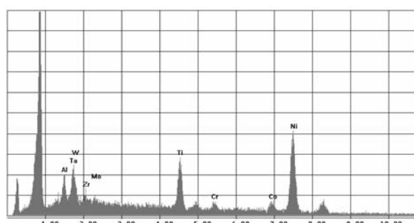
Fig. 8 EDX spectrum of the phase \text{Ni}_3\text{Ti}
