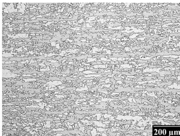
Fig. 1 Microstructure of duplex steels - Uranus 45N and 52N+
