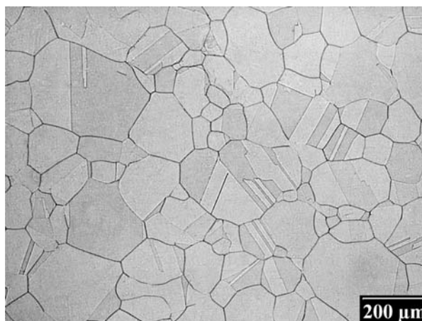
Fig. 2 Microstructure of austenitic steels - Uranus SB8 and B26
