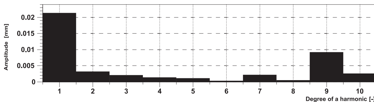
Fig. 6 Amplitude values of separate harmonic parts 1÷10 diagram
