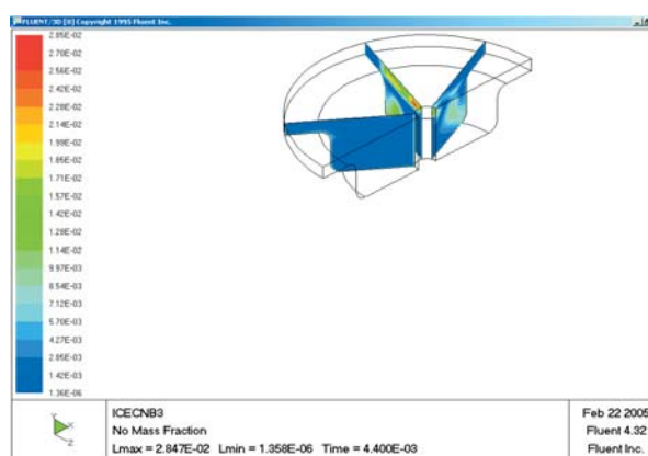
Fig. 6 Mass fraction of NO in the time t = 0.0044 s
