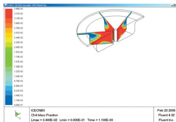
Fig. 5 Mass fraction of CH 4 in the time t = 0.0011 s
