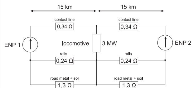
Fig. 8 Substitutional resistance model of single-track railway line
