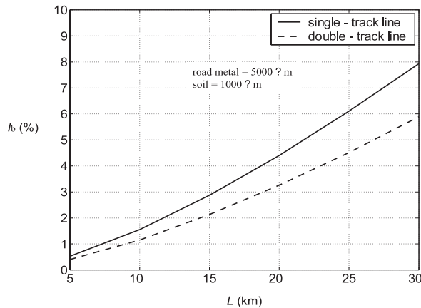
Fig. 6 The amount of stray currents in direct current railway at 3000 V with specific crushed stone resistance of 5000 \Omega\text{m} and specific earth resistance of 1000 \Omega\text{m}
