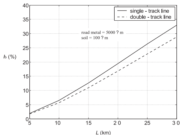
Fig. 4 The amount of stray currents in direct current railway at 3000 V with specific ballast resistance of 5000 \Omega\text{m} and specific earth resistance of 100 \Omega\text{m}
