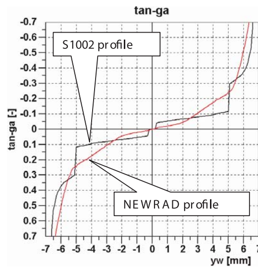
Fig. 13 Tangent gamma function for profiles combination NEWRAD and S1002/UIC60/1:40/1435
