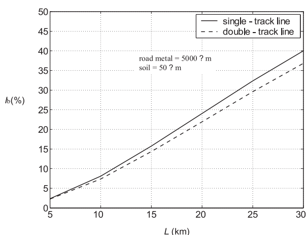
Fig. 3 The amount of stray currents in a direct current railway line at 3000 V with a specific crushed stone resistance of 5000 \Omega\text{m} and a specific earth resistance of 50 \Omega\text{m}
