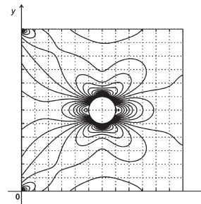
Fig. 8 The strain \varepsilon_x in the x -direction
