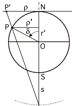
Fig. 8 Satellite projection
