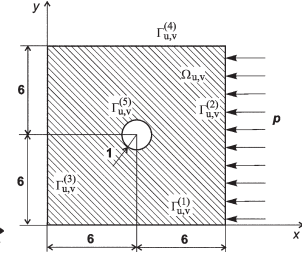
Fig. 5 The domain \Omega_{u,v}
