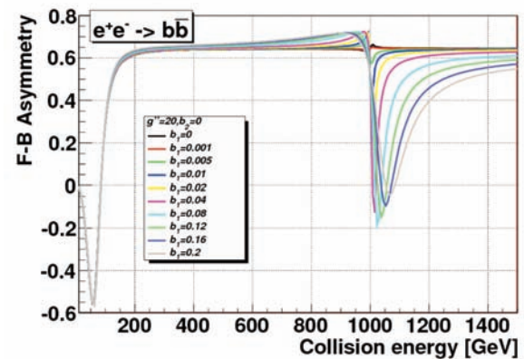
Fig. 6 The forward-backward asymmetry for the process e^+e^- \rightarrow b\bar{b} as a function of the collision energy when M_{V^0} = 1 TeV. While b_2 = 0 the b_1 parameter runs through 0 to 0.2.
