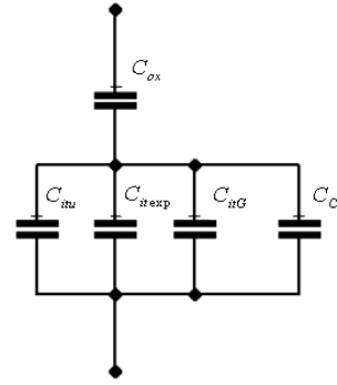
Fig. 2 Equivalent circuit for the MOS structure with interface states. C_{ox} is capacitance of NAOS oxide layer, C_{itu} , C_{it \exp} and C_{itG} are capacitances associated with D_{itu} , D_{it \exp} and D_{itG} , respectively
