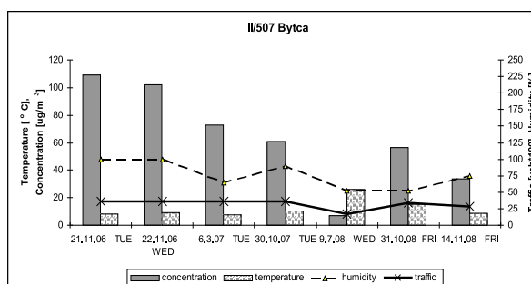
Fig. 5 Long-term observation at the measuring position 2, II/507 road, Bytca bypass
