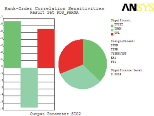
Fig. 5 Sensitivity plot for sigma 2
