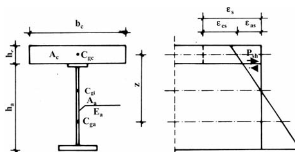
Fig. 2 Dimensions, forces in cross-section and longitudinal layout
