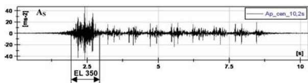
a) The time history of the vertical sleeper acceleration w''_S(t) /the accelerometer A_S - Passage of the locomotive EL 350, t = 2.0 - 3.05 s = 1.05 s.
