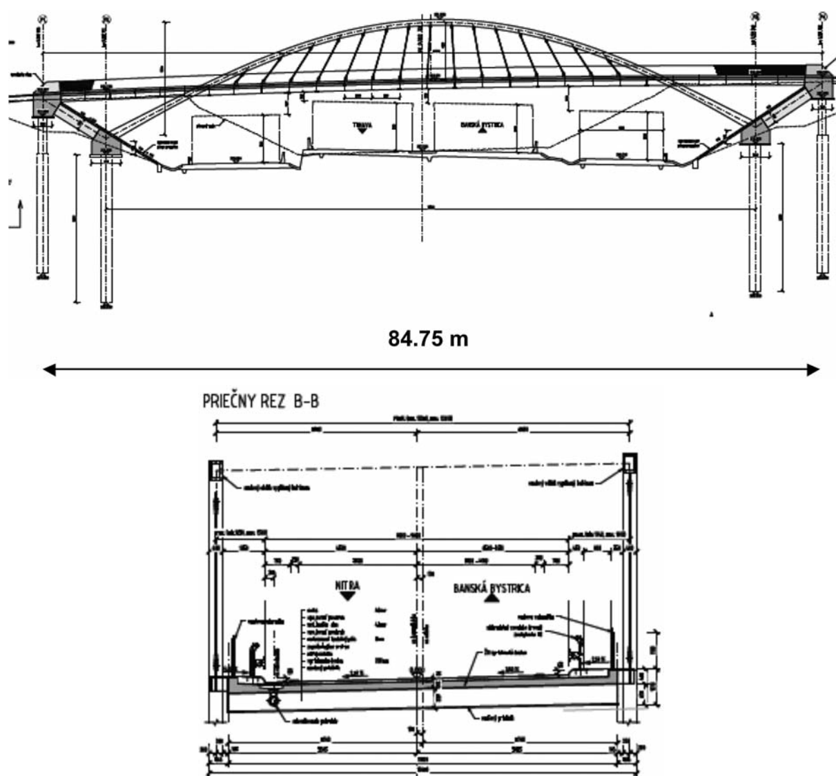
Fig. 1 The bridge model and its cross section – general arrangement.
