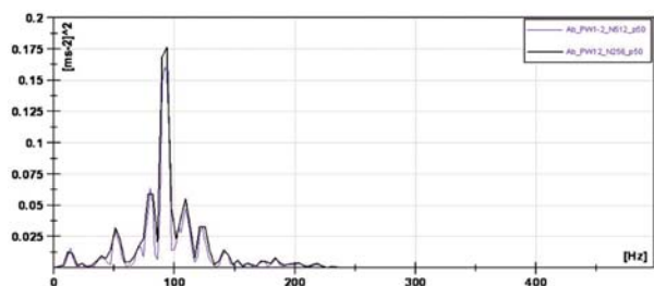
Fig. 10 Analysis of the vertical ballast bed acceleration w''_B(t) /the accelerometer A_B for the passage of coach bogies No. 1-2, t = 3.01 - 3.8 = 0.79 s.
