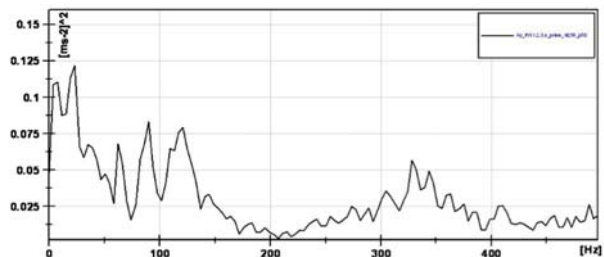
c) b) LABVIEW Analysis: The PWS of the sleeper acceleration w''_s(t) /the accelerometer A_S – The passage of coach bogies No.1-2, No. 2-3, No. 3-4, t = 3.01 - 3.8 = 0.79 s. The mean of 3 PWS, for the three bogies passage: bogies No. 1-2, bogies No. 2-3, bogies No. 3-4. The non-filtering signal for frequencies f = (0 \div 500) Hz).
