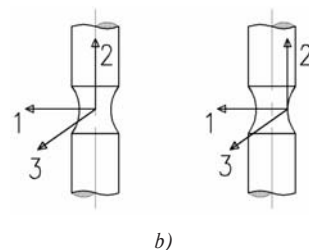
Fig. 2 Specimens used in investigations (a) and notation convention for individual components of strains (b)
