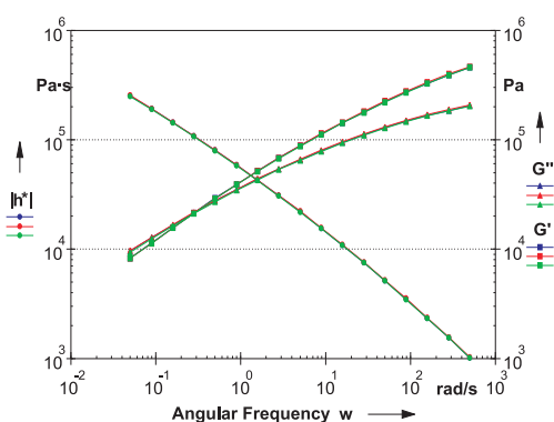
Figs. 4 and 5 Rheological properties of PP and PE 500 exposed in n-hexane for 3 months
