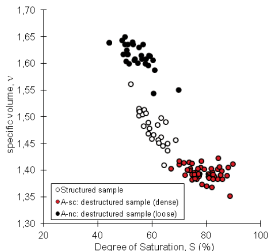
Fig. 1 Specific volume versus degree of saturation of structured and remoulded samples
