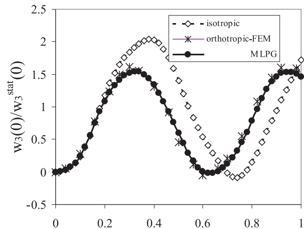
Fig. 4 Time variation of the deflection at the center of a clamped square plate
