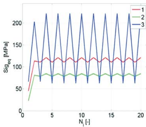
Fig. 10 History of stress convergence for 1 st algorithm
