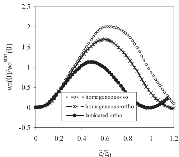
Fig. 5 Time variation of the deflection at the center of a simply supported plates subjected to a suddenly applied load
