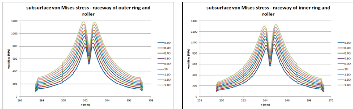
Fig. 9 Dependence of subsurface von Mises stress (outer ring - roller left, inner ring-roller right) on equivalent bearing load
