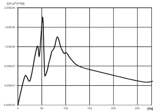
Fig. 4 The input PSD G_{v_j2}(f)
