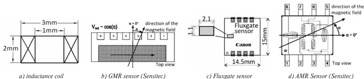
Fig. 3 Sensors layout
