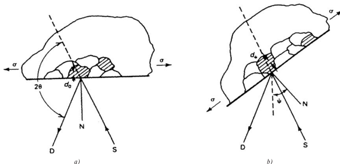
(a) out rotation \psi = 0 . (b) angle of rotation \psi = \psi sample rotated through some known angle \psi , D - detector; S - source; N - normal to the surface.
