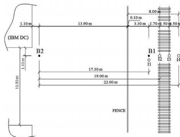
Fig. 5 Accelerometers and ISM (I1- I4) positions and projected building and railway site layout
