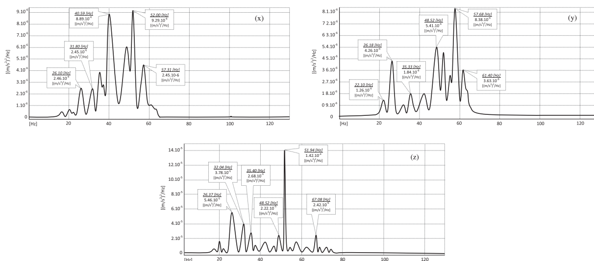
Fig. 11 The input acceleration PSD - G_{11}(f) to foundation at point K1/10 - 130 Hz
