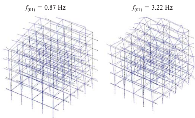
Fig. 10 Structure natural modes
