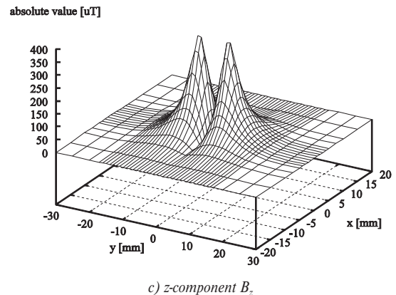
Fig. 6 Absolute values of the sensed magnetic flux density vector B vs. probe position, l_c = 10 mm, d_c = 5 mm, w_c = 0.2 mm, \sigma_c = 0\% of \sigma
