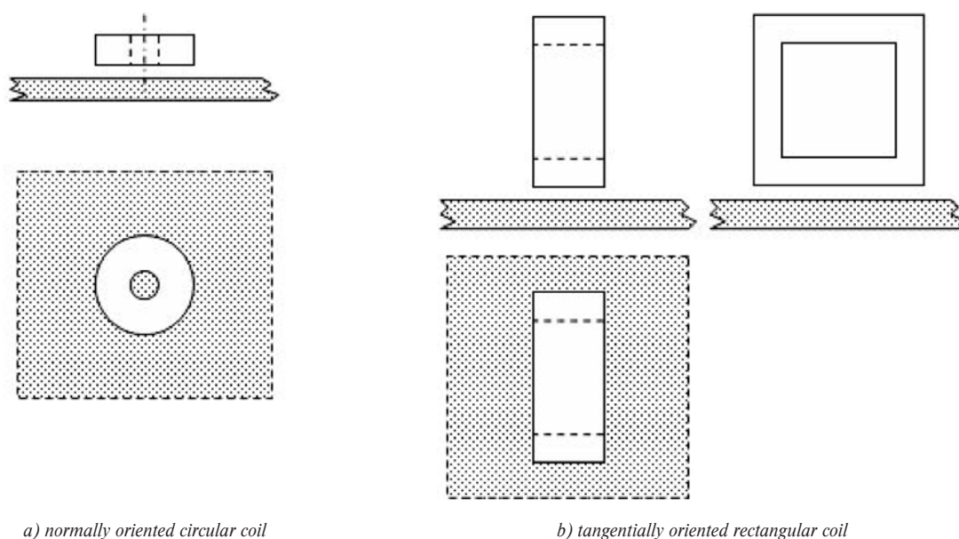
Fig. 1 Basic shapes and orientations of exciting coils
