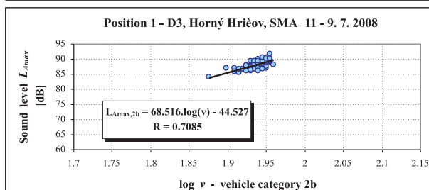
Fig. 1 Regression lines for Position 1
