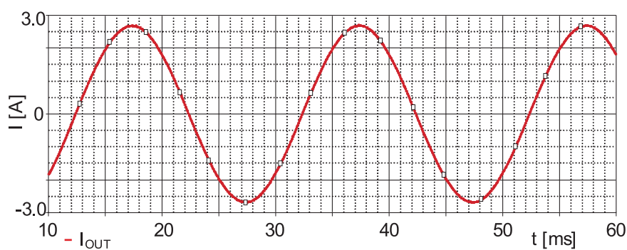
Fig. 5 Simulated waveform of output current of the single-phase converter under R-L load ( U_{DC} = 350V , R = 10 \Omega , L = 30 mH , f_{SW1} = 10 kHz , f_{SW2} = 20 kHz , f_{OUT} = 50 Hz )
