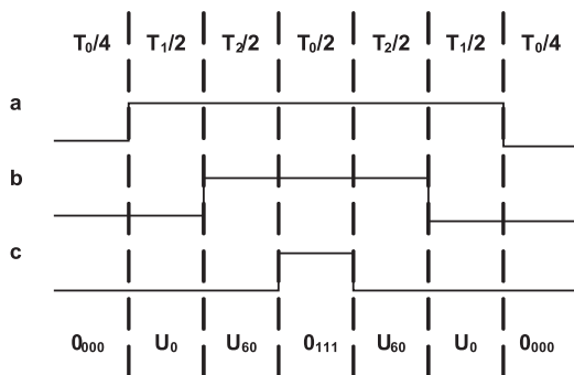
Fig. 2 Switching times assignment of the upper transistors in first sector during PWM period [1]
