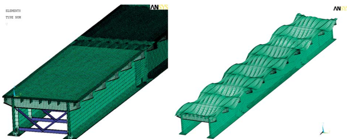
Fig. 1 Structural model of bridge with orthotropic plate deck - detail of finite element meshing and shape of initial imperfections (100 times multiplied)
