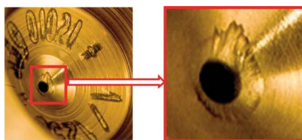
Fig. 4. Damaged steering valve socket in a new injector after the work with the constant contaminants in the fuel
