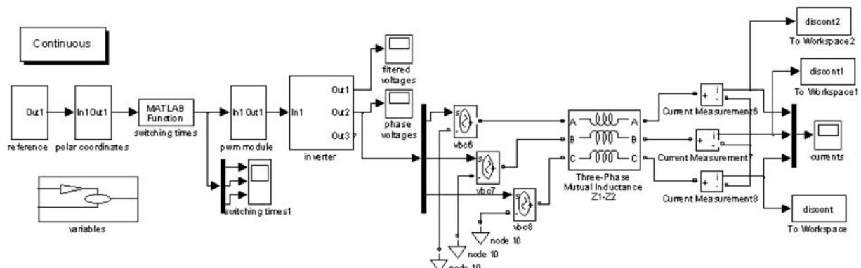
Fig. 6 Simulating scheme
