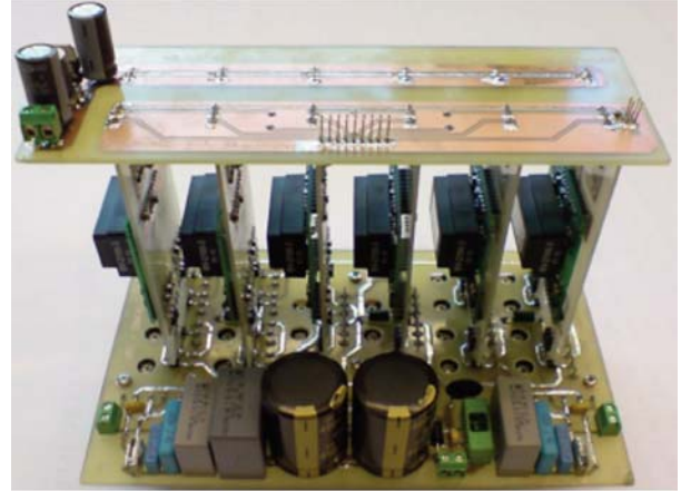
Fig. 8 Photography of complet two phase two stage converter with high-frequency AC link and ortogonal output
