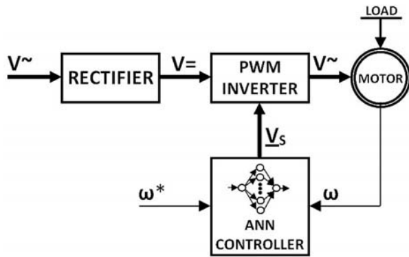
Fig. 1 ANN induction motor control scheme
