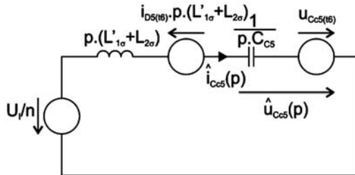
Fig. 13 Equivalent operator circuit for interval t_6 - t_7
