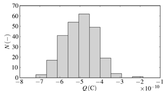
Fig. 5 Distribution of charges of the PVC particles
