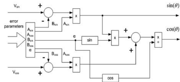
Fig. 5 Correction block
