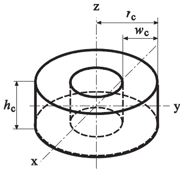
Fig. 2 Layout of circular exciting coil
