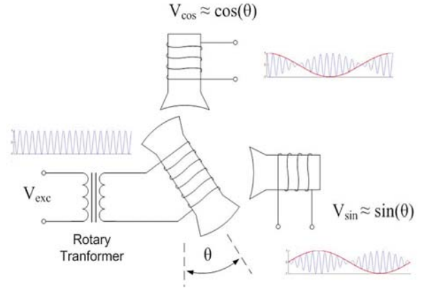
Fig. 2 Resolver schematics
