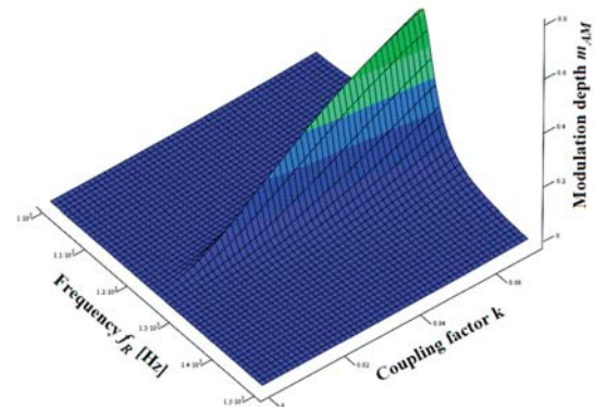
Fig. 8 Modulation depth m_{AM} as a function of coupling factor k and resonant frequency f_R of reader antenna
