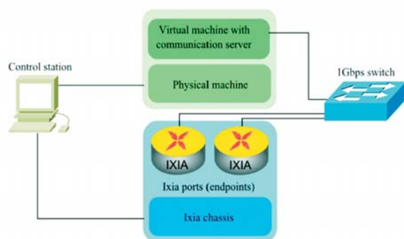
Fig. 1 Test topology
