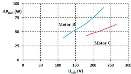
Fig. 14 The simulated iron losses of Motors B and C
