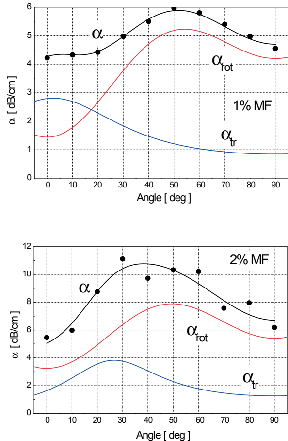
Fig. 4 Development of rotation and translation part of acoustic attenuation and their sum measured in the 1% and 2% MF based on MOGUL for temperature 20 °C
