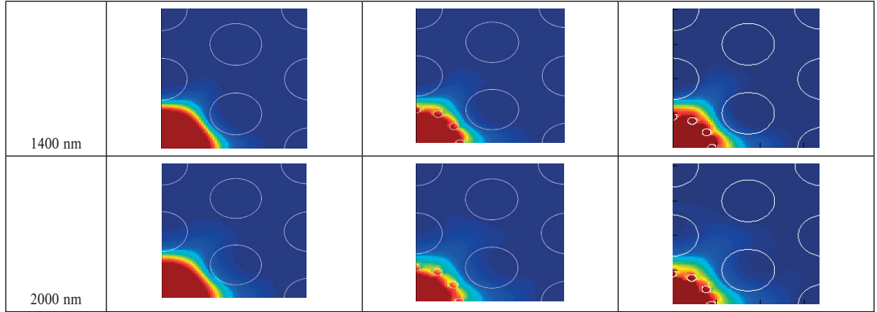
Fig. 2 Mode distributions of z -component of Poynting vector for PCFs with constant d_n = 200 nm, but radius of rings L_n = 1000 nm and 900 nm for different wavelengths of light.
