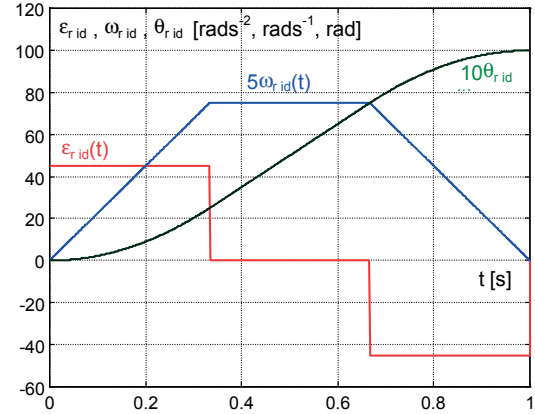
Fig. 4 Energy saving control, trapezoidal speed profile
