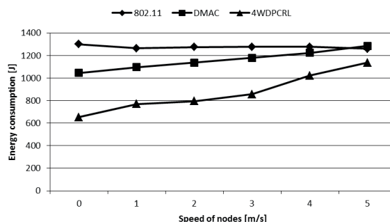
Fig. 10 Average values of energy consumption of all nodes for different MAC algorithms and for 10 data flows
