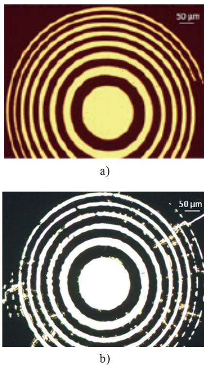
Fig. 4 Optical microscope image of FZP structure prepared on a) glass and b) PDMS surface
