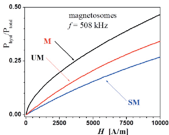
Fig. 8 Proportion of hysteresis processes to total losses
