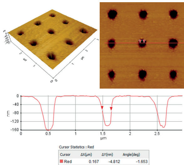
Fig. 3 AFM image and line profile analysis of prepared periodic structure with 1 \mu m period in both directions and air hole FWHM app. 170 nm
