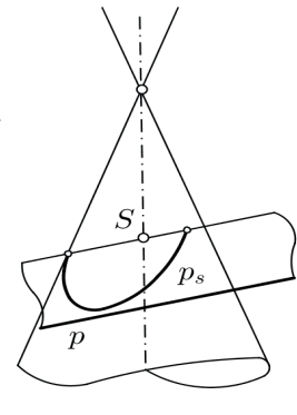
Fig. 22 Skew lines o, p
