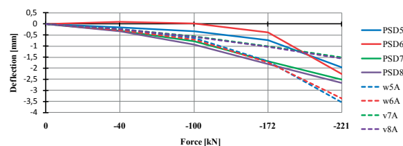
Fig. 6 Comparison of horizontal deflections in the cross-sections of sample C1
