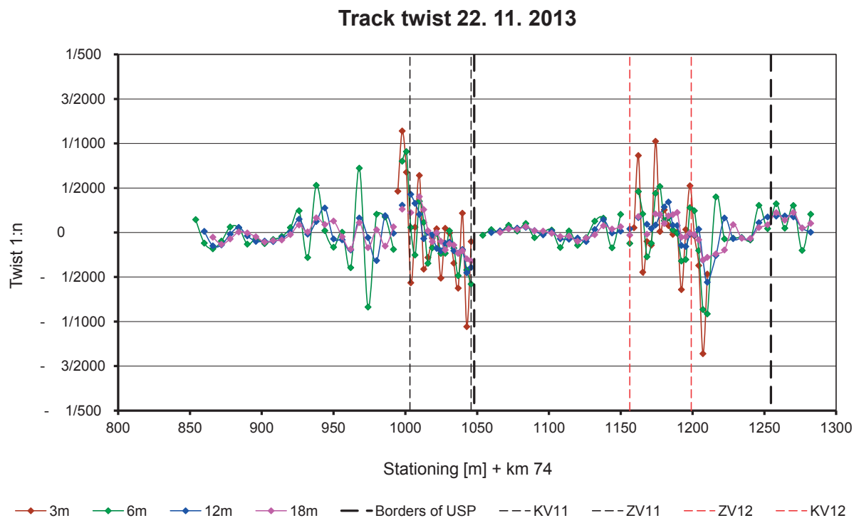
Fig. 4 Track twist in Plana nad Luznici over the length of 3 m, 6 m, 12 m and 18 m; 22 November 2013
