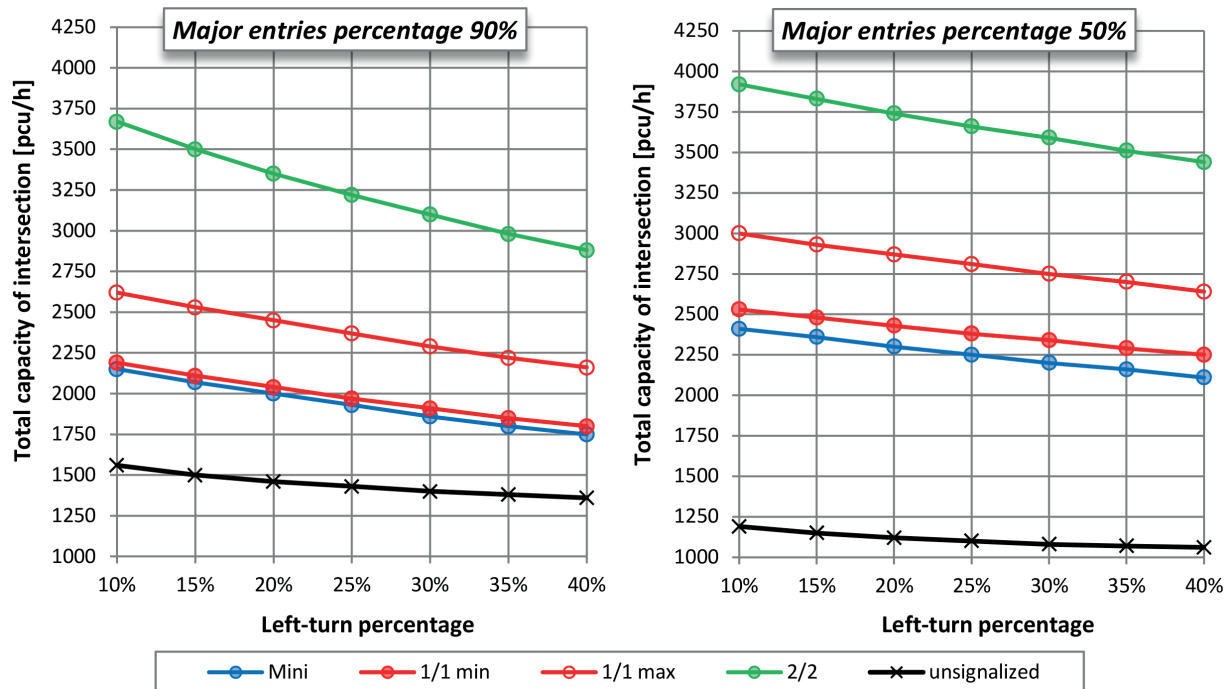
Fig. 5 Total capacities of roundabouts and unsignalized intersection depending on proportion of left-turn vehicles
