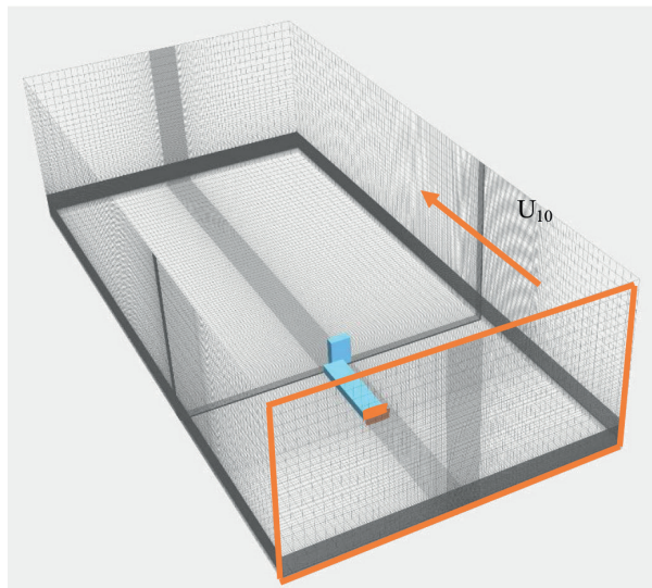
Fig. 1 Computational domain with dimension 775 \times 1600 \times 420 m and marked investigated windward facade, inlet plane with flow direction and wind velocity U_{10} = 10 m/s
