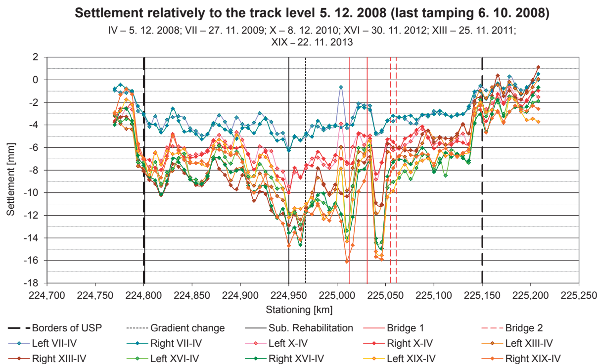
Fig. 5 The track settlement in Havlickuv Brod – Okrouhlice test track section after track tamping relatively to the track level of the 5 December 2008
