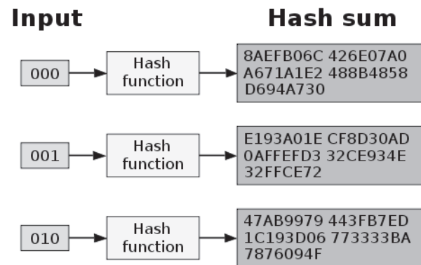
Fig. 1 Avalanche effect for SHA-1 [8]
