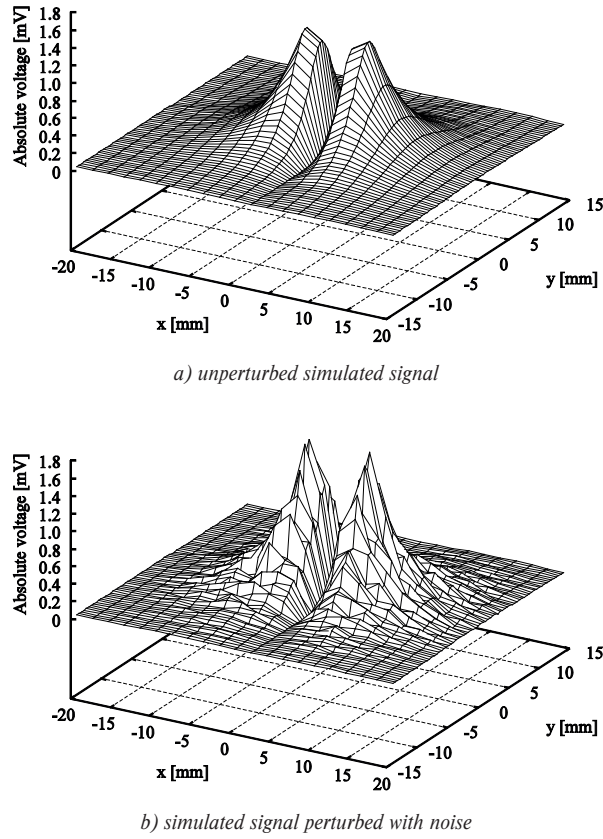
Fig. 4 Simulated ECT response signal
