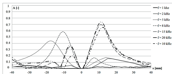
Fig. 12. Experimental results: inductance sensor, SC crack (load force F = 1.8 kN, t = 6 hours)
