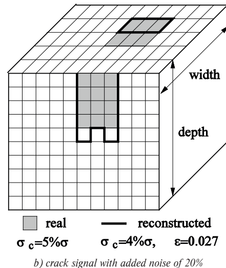
Fig. 5 Reconstruction of a partially conductive crack, crack model 2
