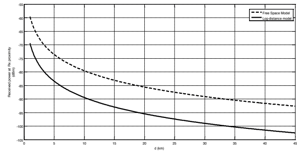
Fig. 2. Local mean value of received power as a function of distance
