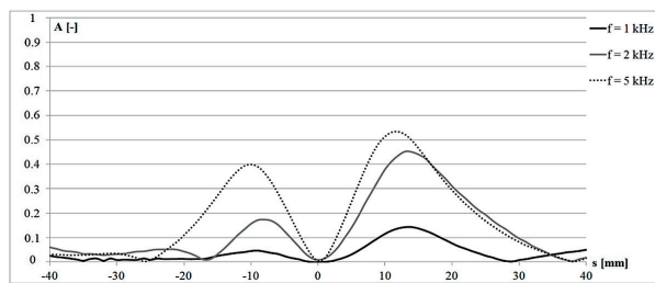
Fig. 10. Experimental results: fluxgate sensor, SC crack (load force F = 1.2 kN, t = 12 hours)
