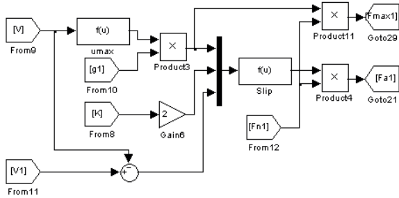
Fig. 5 Adhesion model in MATLAB - Simulink
