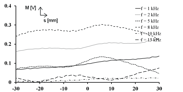
Fig. 16. Experimental results - AMR sensor (left), SCC crack (load force F=1.8 kN, t=12 hours)
