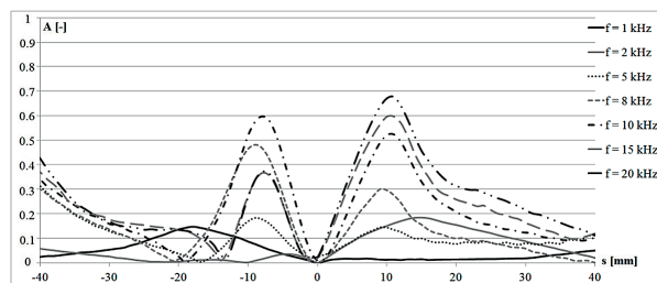
Fig. 11. Experimental results: GMR sensor, SC crack (load force F = 1.8 kN, t = 6 hours)
