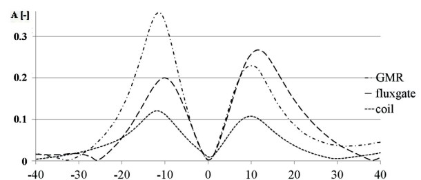
Fig. 17. Experimental results: SC crack, (load force F = 1.2 kN, t = 24 hours), excitation frequency f = 1 kHz
