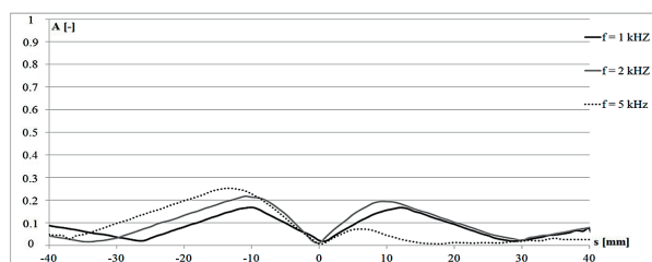
Fig. 13. Experimental results: fluxgate sensor, SC crack (load force F = 1.8 kN, t = 6 hours)
