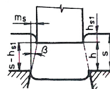
Fig. 9 Determining the cutting gap size
