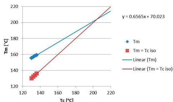
Figure 7 Determination of the equilibrium melting temperature
