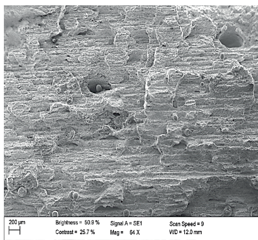
Figure 9 Woody fracture
