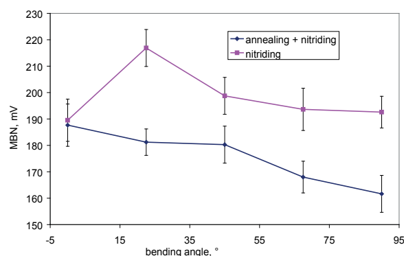
Figure 11 MBN versus the bending angle - outer surface
