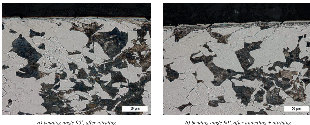
Figure 5 Metallographic images of the outer surface
