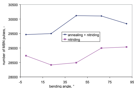
Figure 12 MBN pulses versus the bending angle - the inner surface
