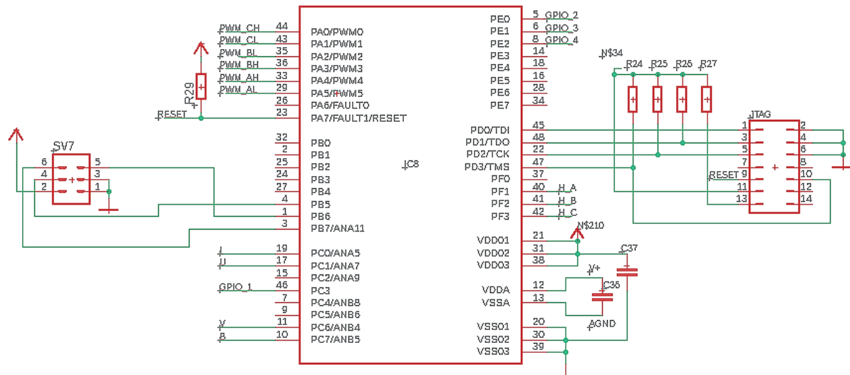
Figure 7 Controlling processor
