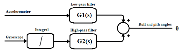
Figure 6 Complementary filters with constant gain
