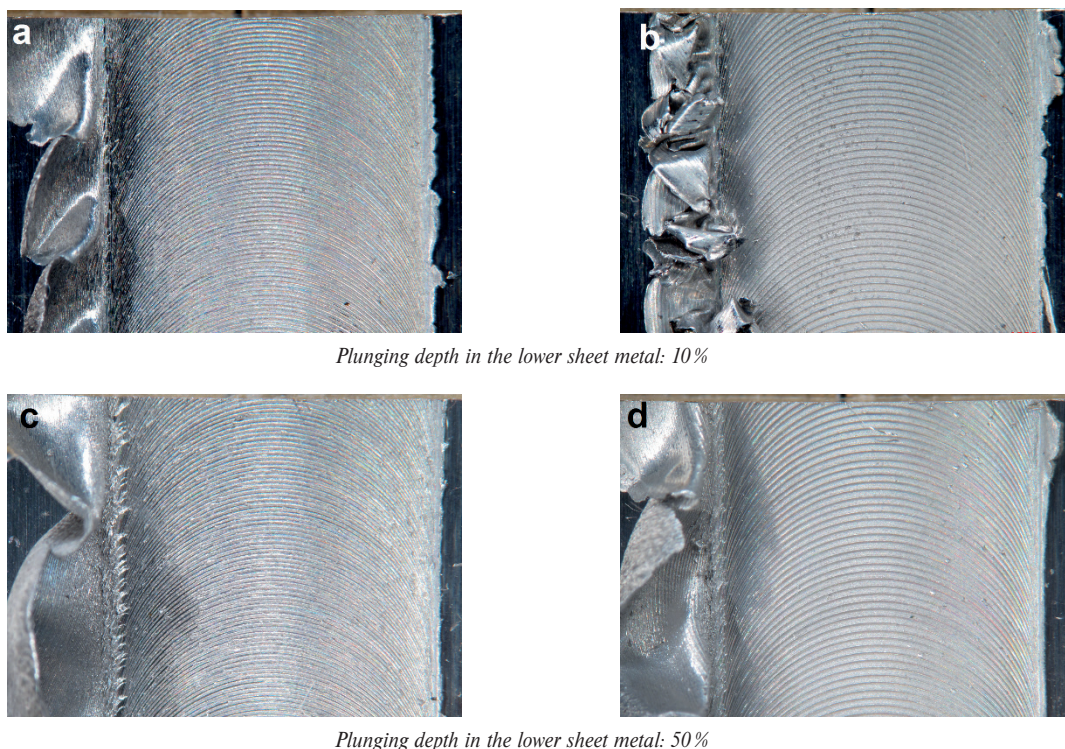
Figure 2 Weld face view of the FSW joints prepared using tool pin plunge depth of 10 % and 50 % and process parameters: a, b) \omega = 700 \text{ rpm} ; v = 100 \text{ mm min}^{-1} , c, d) \omega = 1300 \text{ rpm} ; v = 300 \text{ mm min}^{-1}
