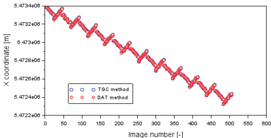
Figure 2 Values of the projection centre X coordinate based on TGC and DAT methods
