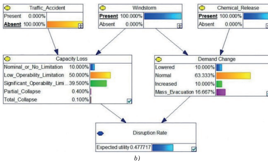
Figure 5 The ID model for calculation of the Disruption rate for two (present) threats combination
