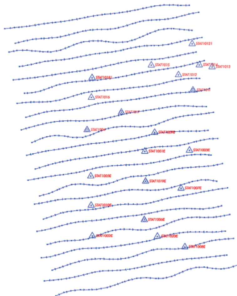
Figure 1 Visualization of the test photogrammetric block - altitude 150 m
