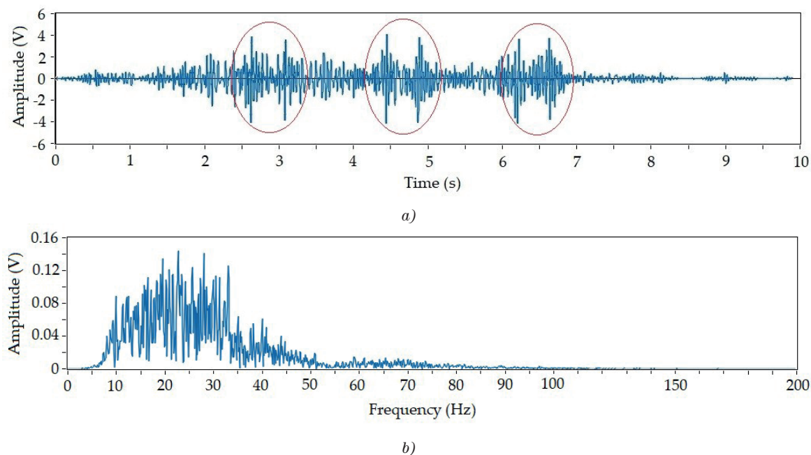
Figure 7 Passage recording for tram vehicle with 3 axles / 6 wheels (type Stadler Tango NF2); a) time record b) frequency record
