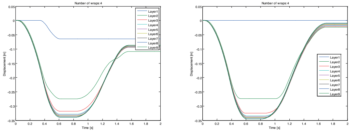
Figure 10 Comparison of the displacements of layers (4 wraps, variant 1 left and variant 2 right)
